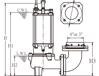
ECT-SE W/Elbow For 5HP & 7.5HP-3"/4"
