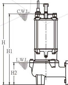
ECT-S For 2HP & 3HP-2"/3" For 5HP & 7.5HP-3"/4"
