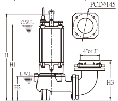
ECT-VE W/Elbow For 5HP & 7.5HP -3"4"
